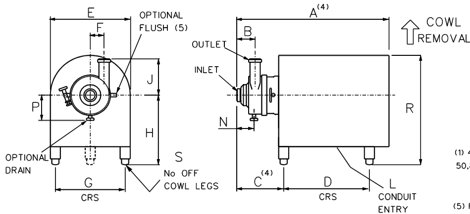
COWLED PUMP
