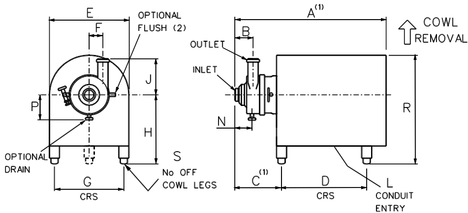
COWLED PUMP
