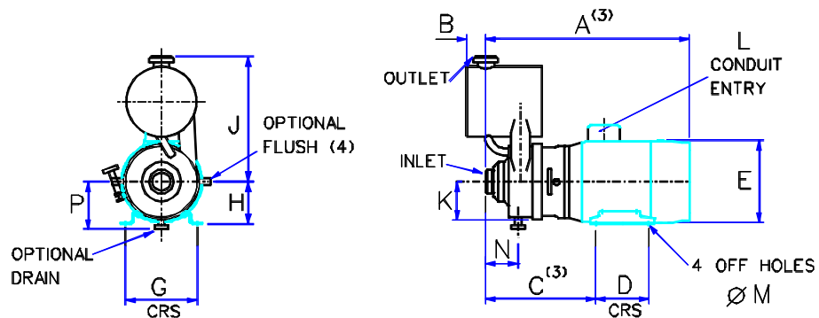
STANDARD PUMP
