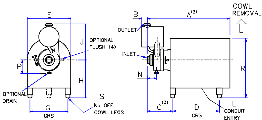
COWLED PUMP
