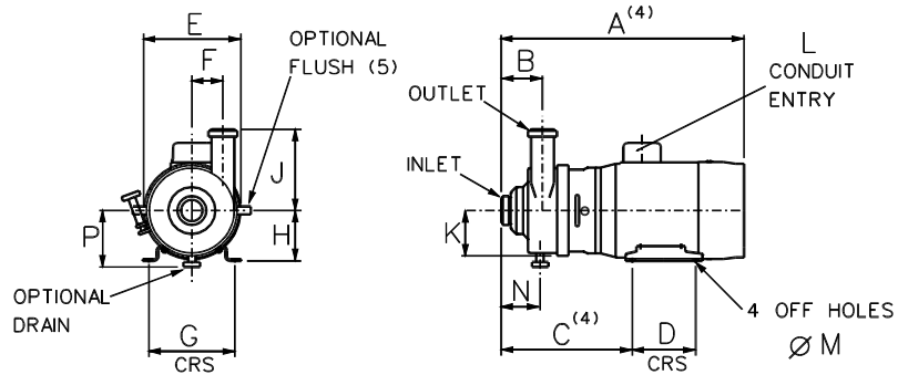
STANDARD PUMP
