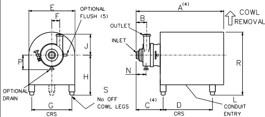
COWLED PUMP
