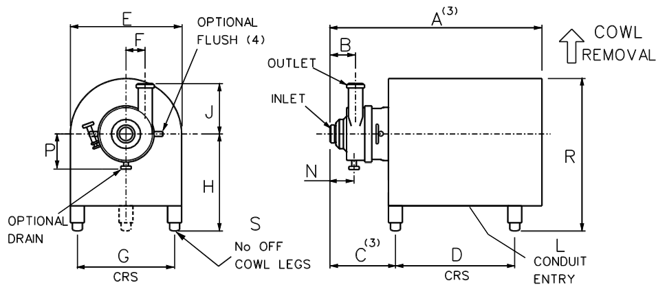
COWLED PUMP
