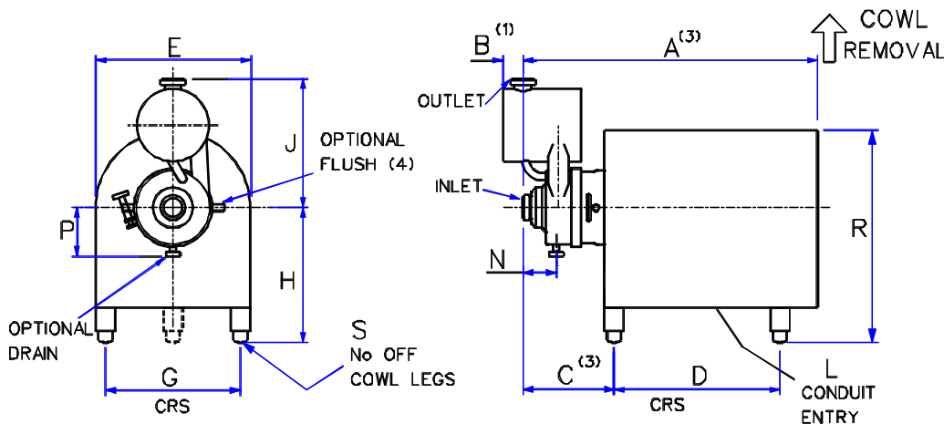
COWLLED PUMP
