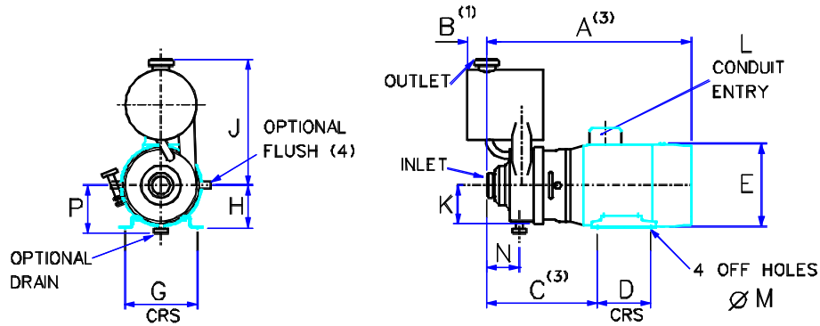
STANDARD PUMP
