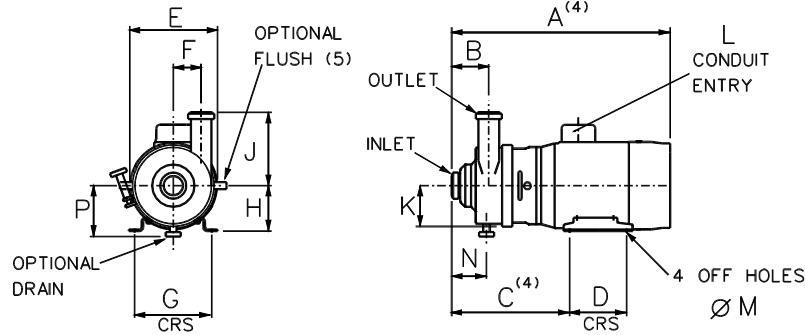
STANDARD PUMP
