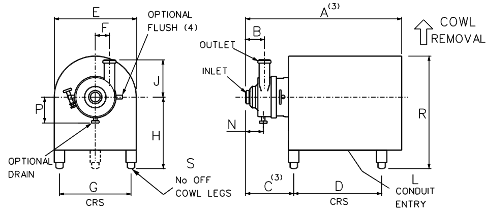
COWLED PUMP
