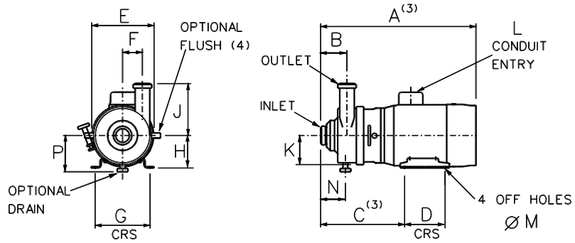
STANDARD PUMP
