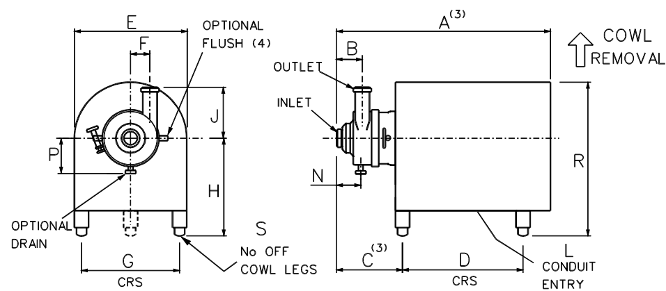
COWLED PUMP
