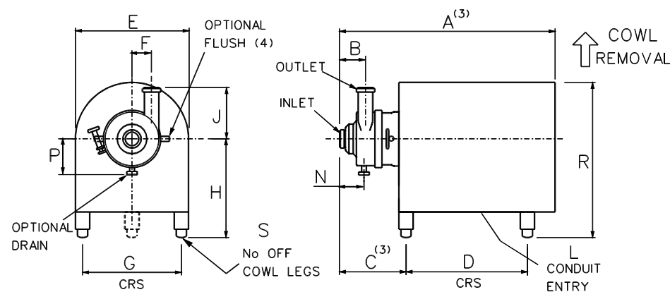
COWLED PUMP
