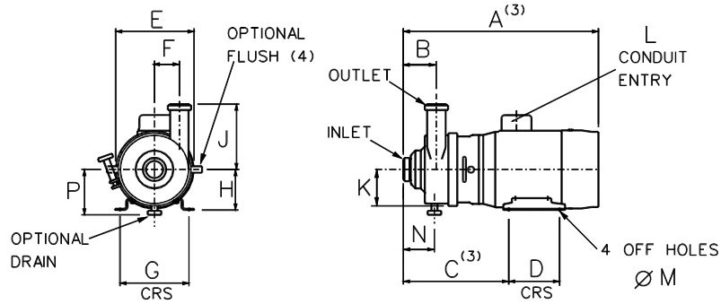
STANDARD PUMP
