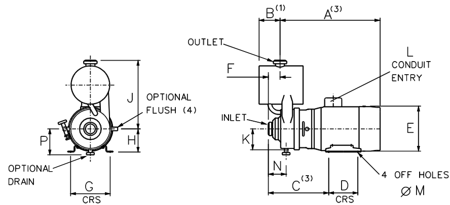
STANDARD PUMP
