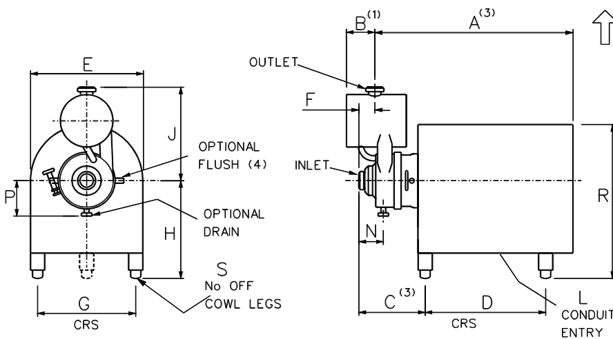
COWLED PUMP
