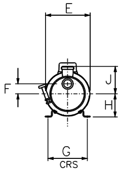
STANDARD PUMP
