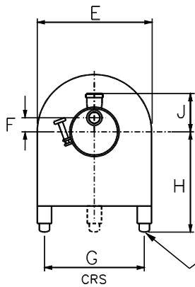
COWLED PUMP
